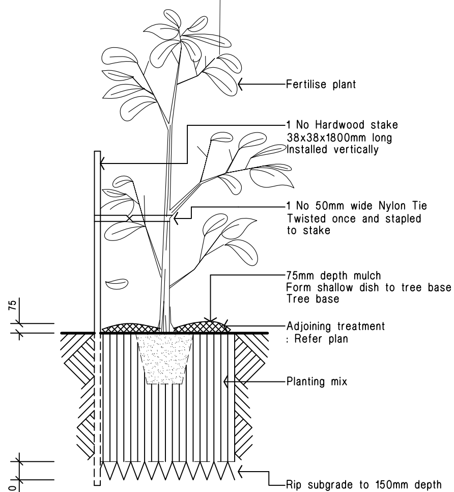
15 - 35 litre Tree planting Detail. Not To Scale.
